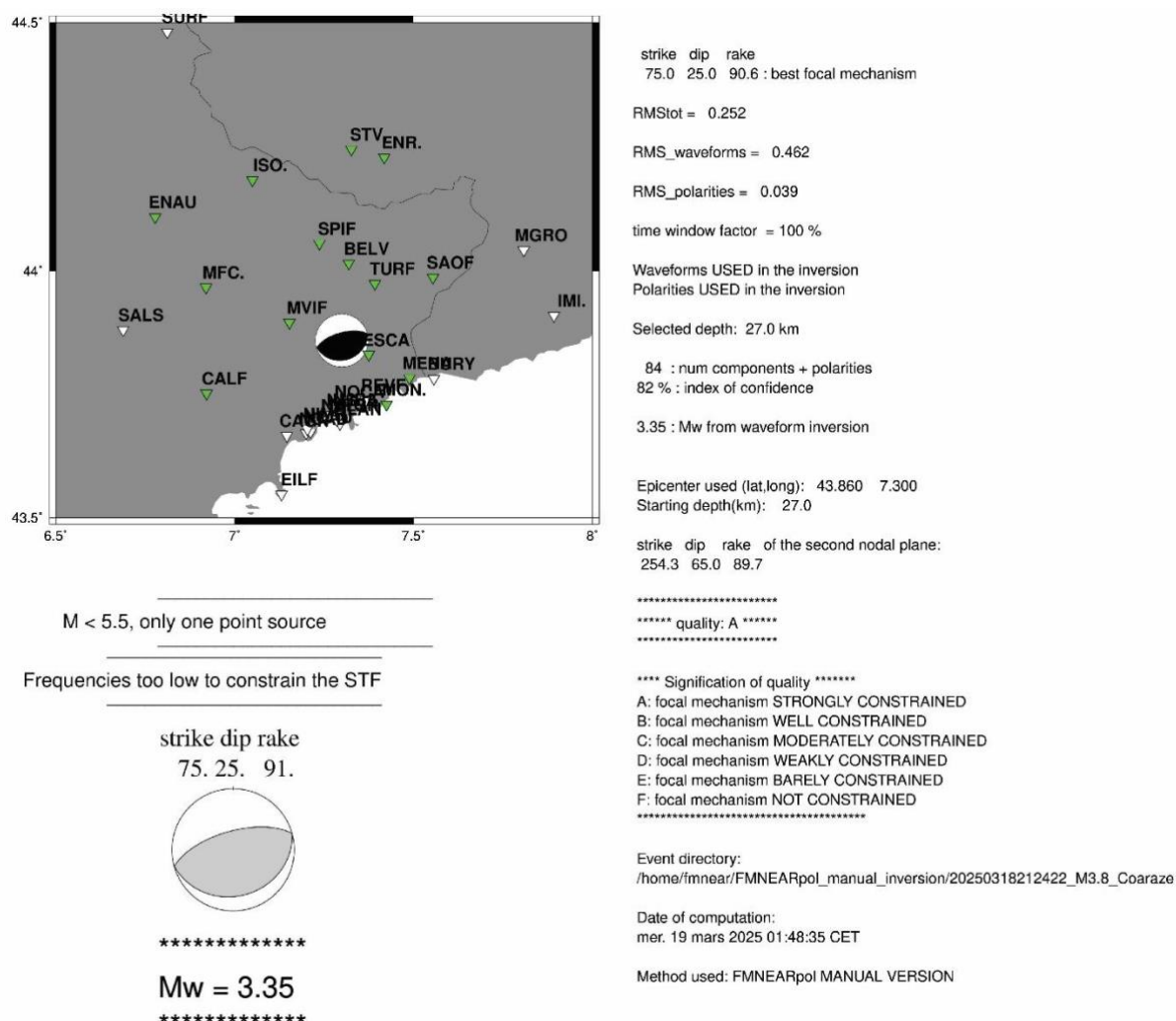
Figure 1-2 Mécanisme au foyer (B. Delouis, Géoazur)
