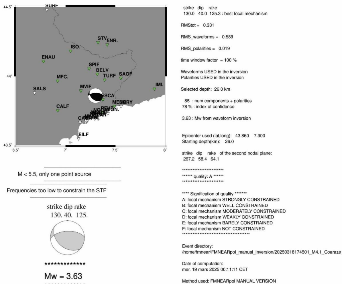
Figure 1-1 Mécanisme au foyer (B. Delouis, Géoazur)
